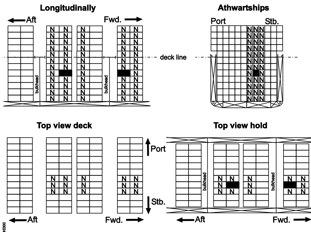
1 – Situation open versus open – UNDER DECK Note: All bulkheads and decks shall be resistant to fire and liquids.
